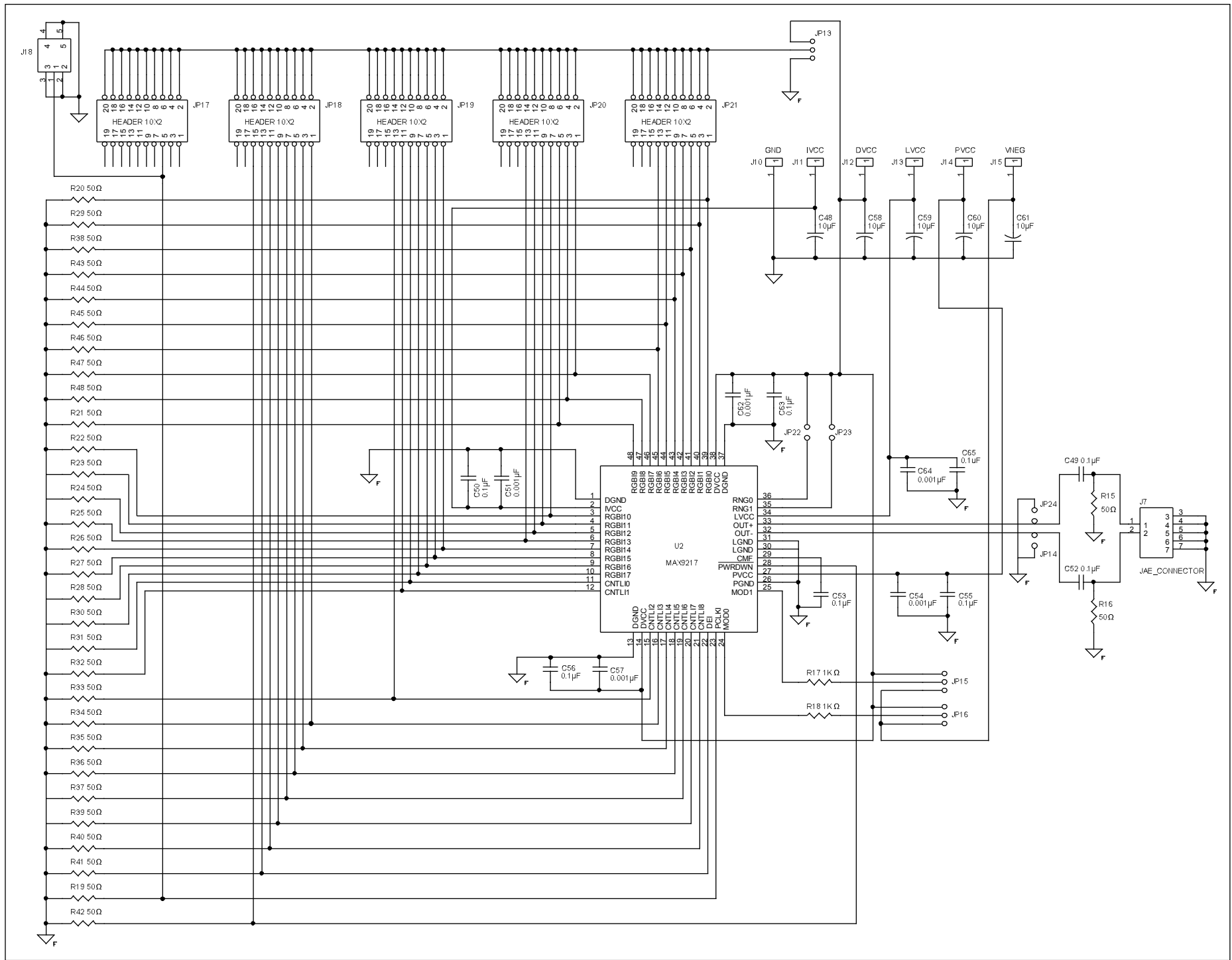
Figure 1. Circuit schematic for the MAX9217 EV Kit.
