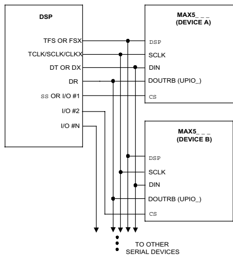
DSP FRAME SYNC MODE 8-BIT CONTROL DATA READ (2 DEVICES):
