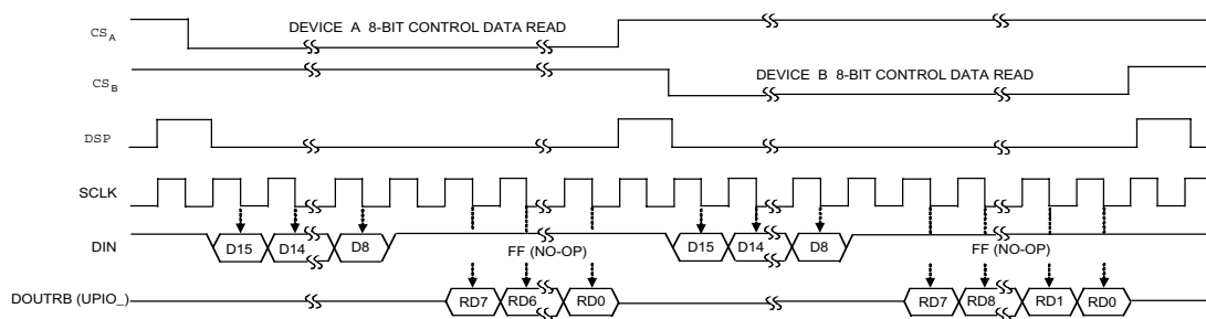
DSP FRAME SYNC MODE 8-BIT CONTROL DATA READ (2 DEVICES):
