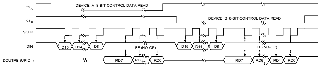
SPI (CPOL=1, CPHA=1) 8-BIT CONTROL DATA READ (2 DACS):
