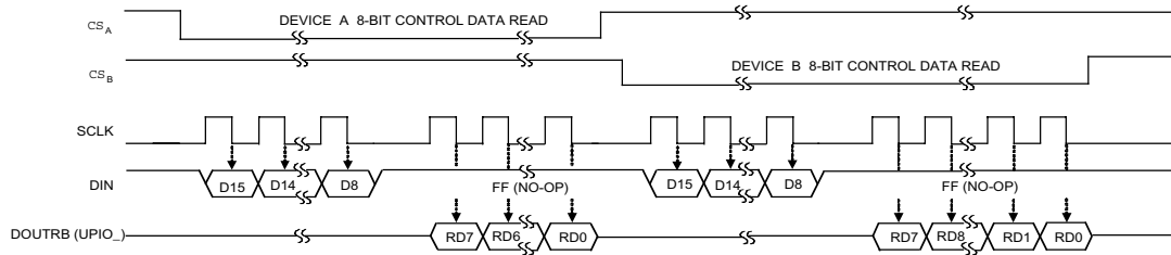
SPI (CPOL=0, CPHA=1) 8-BIT CONTROL DATA READ (2 DACS):
