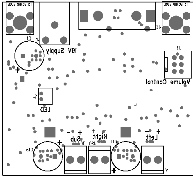
PCB: BOTTOM SILCScreen
