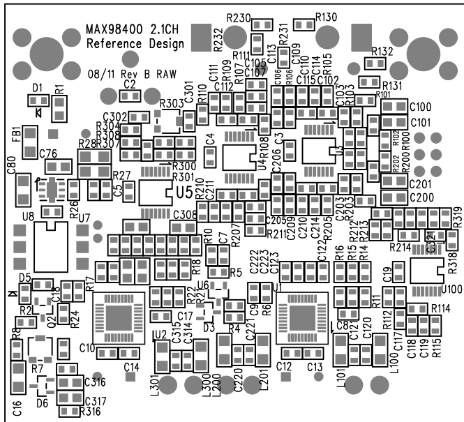
PCB: TOP SILCScreen
