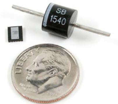
Figure 9. Solar cell optimizer IC from Maxim Integrated.
