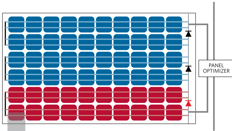
Figure 1. Performance of conventional module vs. solar cell optimizer module, when a single cell is shaded.
