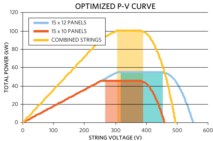
Figure 6. Performance gained when uneven strings are connected in parallel.
