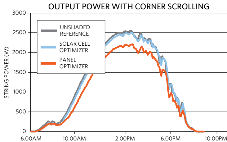
Figure 8. Performance of cell optimizer vs. module optimizer with uniform soiling pattern (as in Figure 7).
