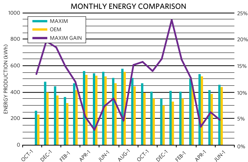
Figure 5. Performance chart of a side-by-side comparison, with and without solar cell optimizers.
