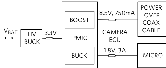
Figure 4. Power PMIC Inside the Camera ECU
