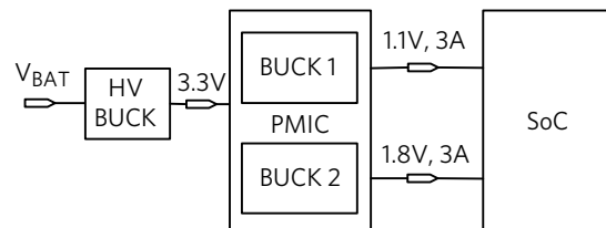
Figure 5. Instrument Cluster PMIC
